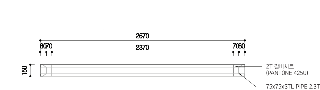
1 TOP VIEW 088 SCALE : A3 1/25
