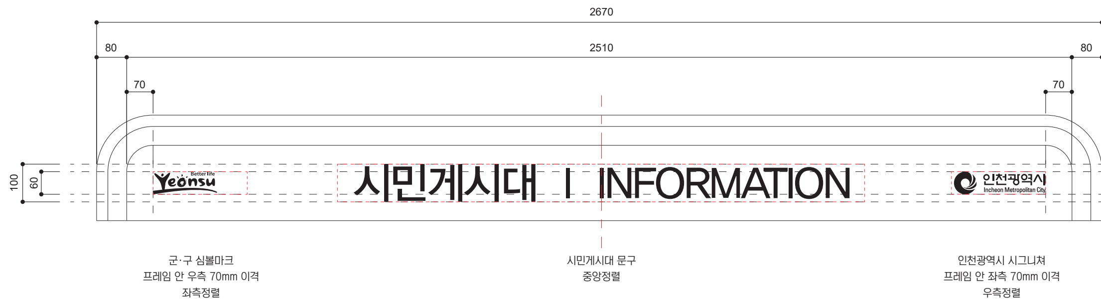
1 FRONT VIEW 089 SCALE : A3 1/10
