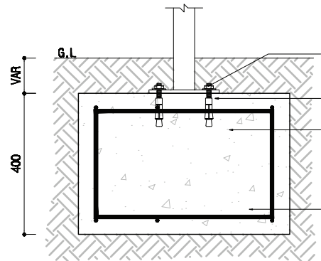
7 DETAIL B 088 SCALE : A3 1/10
